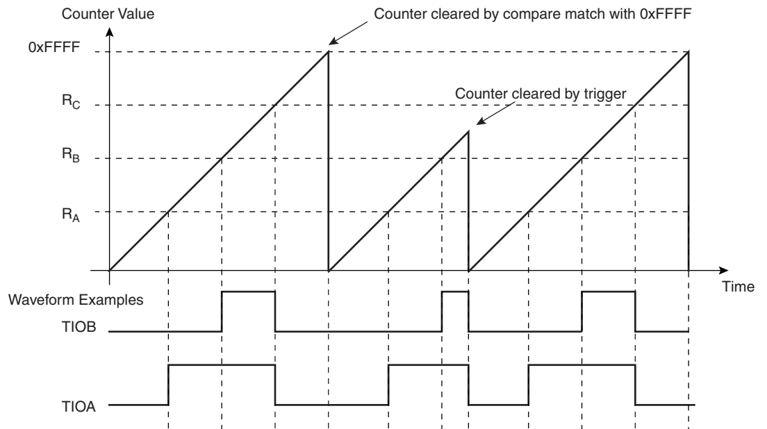
Figure 31-7. WAVSEL= 00 with trigger
