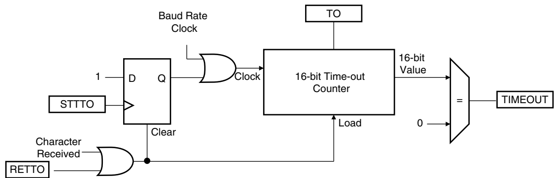
Figure 30-14. Receiver Time-out Block Diagram
