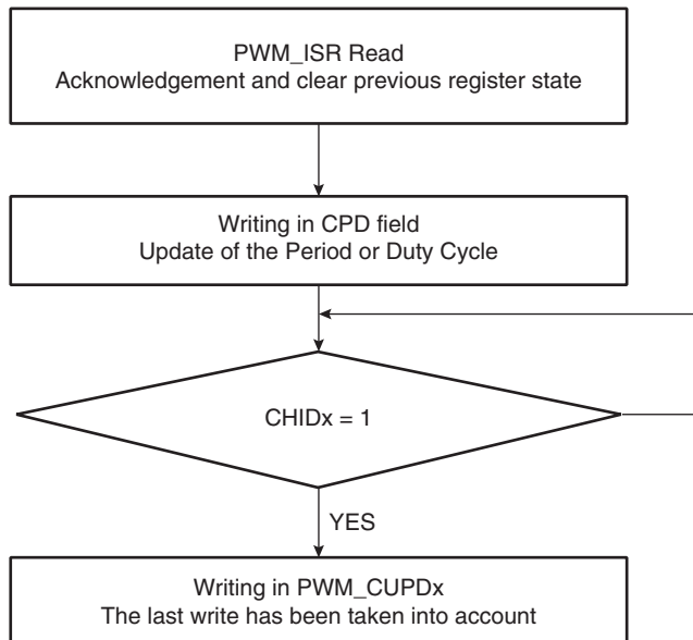
Figure 32-7. Polling Method
